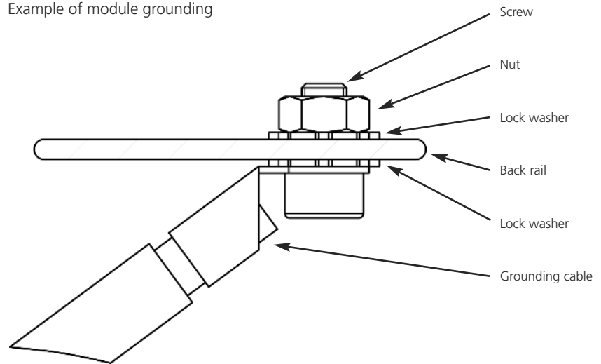
Example of module grounding
